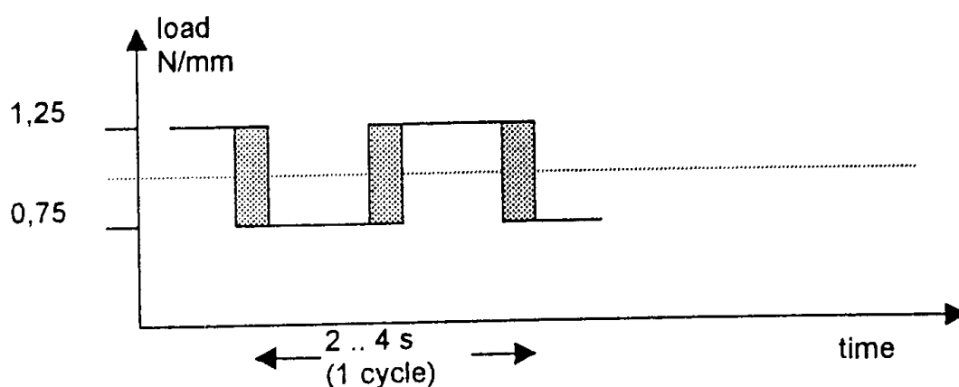
Figure 7 - Loading cycle
