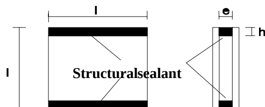
Figure 17 - Sample geometry
